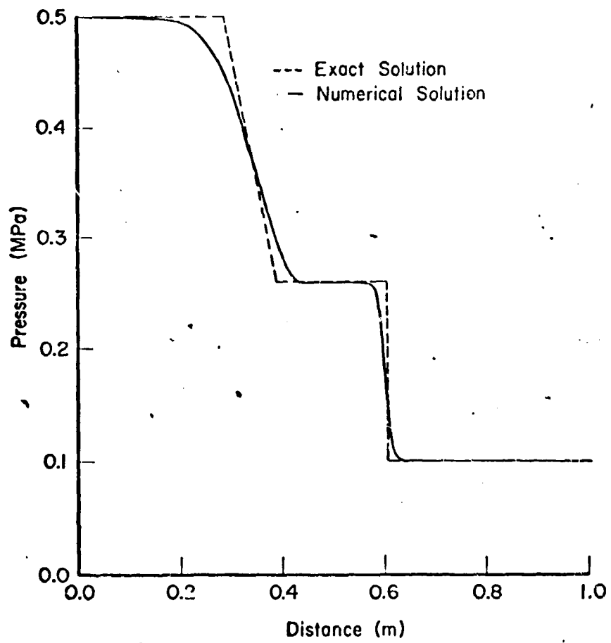
Fig. 3.3b. Pressure at t = 2 \text{ ms} for \delta t = 100 \mu\text{s} , \delta z = 2.5 \text{ mm} without phase change.
